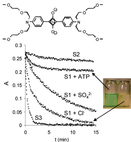
Figure 1. Absorbance at 643 nm (squaraine band) vs time at pH 5 for solids S1 in the presence of ATP, chloride, or sulfate (0.01 M) and S2 and S3 in the presence of ATP (0.01 M) in water/acetonitrile 90:10 v/v. The figure also shows a scheme of the used squaraine dye and a photograph of the S1 -ATP and S1 -chloride systems after 15 min of reaction.
